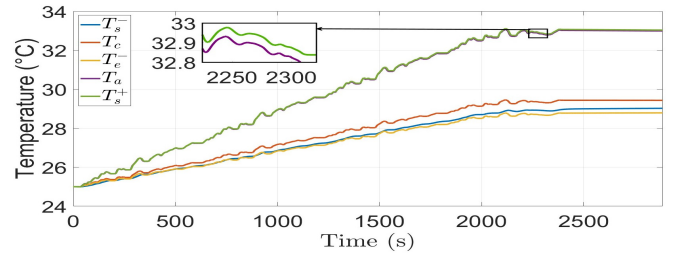
Fig. 4: Temperatures in different regions of the ASSB.
