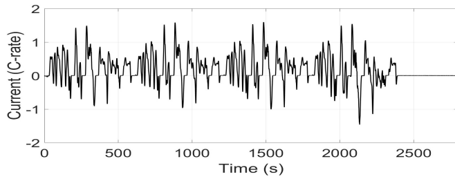
Fig. 2: Current profile used in the UDDS simulation.
