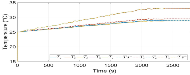
Fig. 6: Comparison of true and estimated temperature states in the ASSB.
